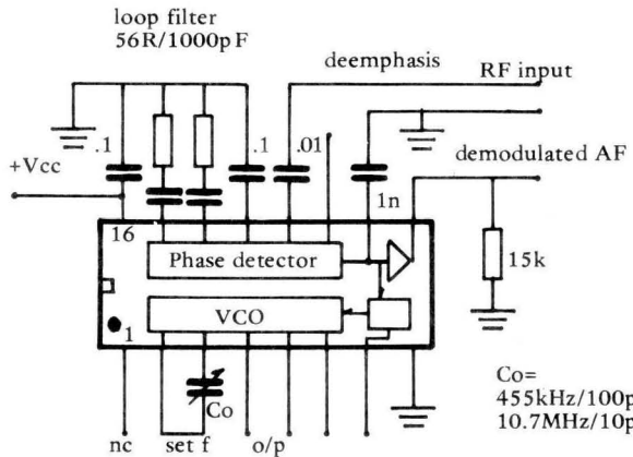
Figure 1. NE560B used as an FM demodulator. PLL ICs make excellent communications demodulators, but inherent noise makes them unsuited to local broadcast conditions, where the HA1137W etc. are superior amplifier and decoders.
