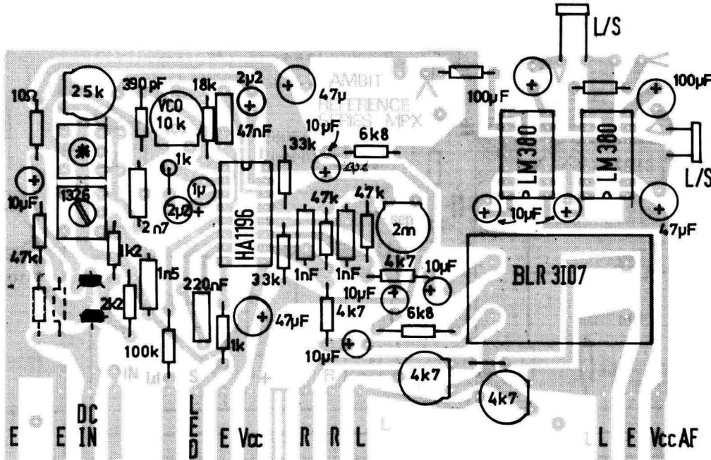
Component layout, viewed from underside
