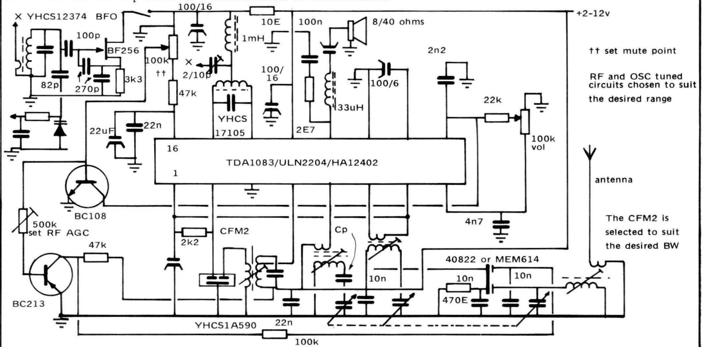
Figure five: An AM/SSB application
