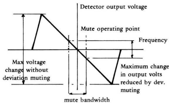
Detector 'S' (or 'Z') curve for a strong signal
