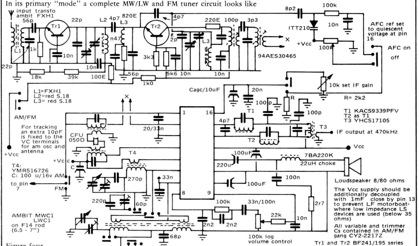
Figure four The complete Broadcast receiver
