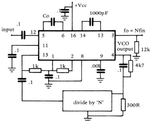
Figure 3. NE562B used in its synthesis application, in conjunction with an external programmable counter. (8281 etc.)
