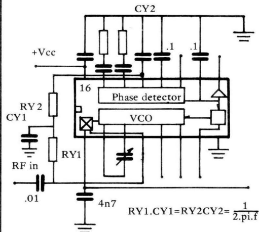
Figure two. The NE561B AM synchronous detector
