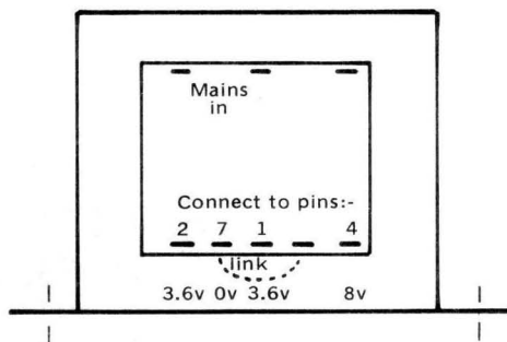
Mains Transformer Connections
