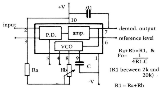
Figure 4. The NE565A as an FM demodulator for FSK, offering increased output over the 560/1/2, but at a lower frequency.
