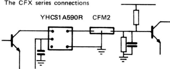
The CFX series connections
