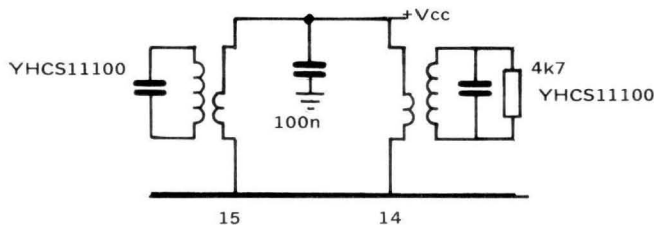
Figure 6: Detector arrangement for NBFM operation
