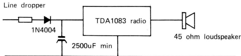
Figure three: The mains dropper system
