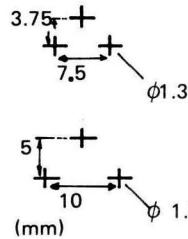
PCB drilling detail
