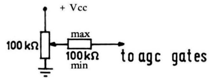
Manual IF AGC control
