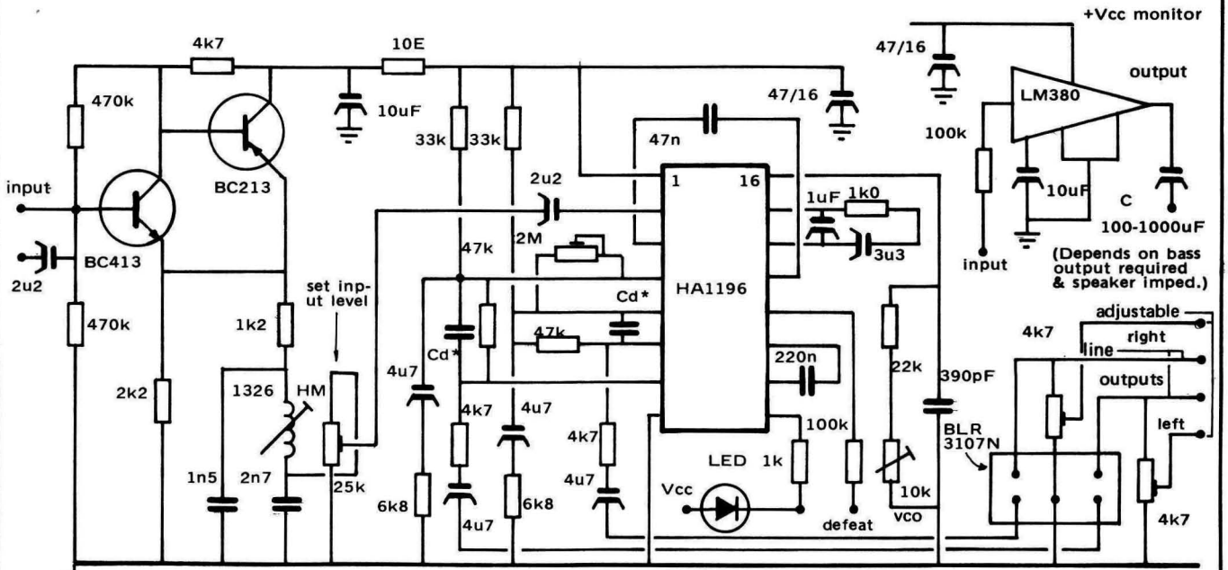
Monitor PA circuit (x2)
