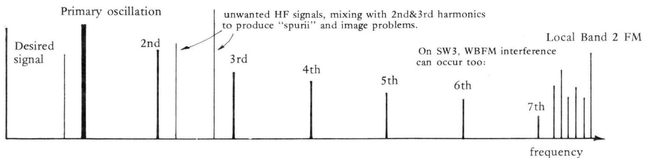
Figure four: A spectral consideration of SW mixing and spuri problems
