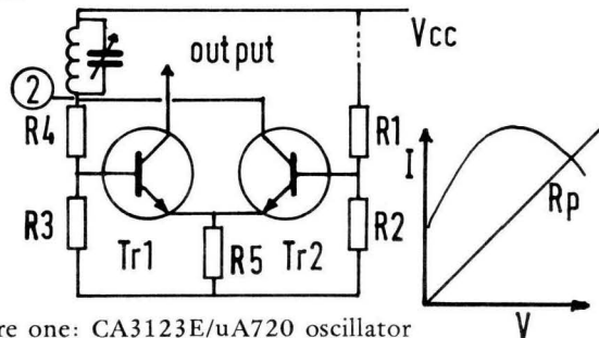
Figure one: CA3123E/uA720 oscillator
