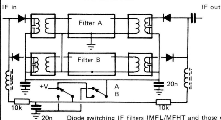
Diode switching IF filters (MFL/MFHT and those with input/output IFs)
